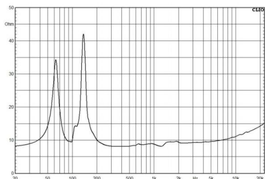
Impedance Curve (Constant Impedance)
